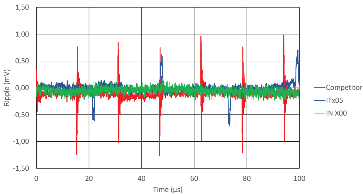
Figure 7: Ripple waveform with a 10 \Omega burden on a scope
