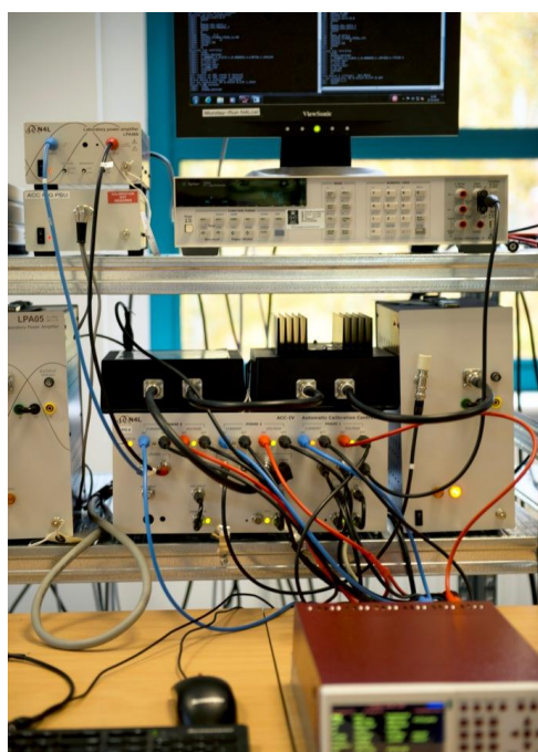
N4L: 10mHz to 2MHz Sinewave Calibration
