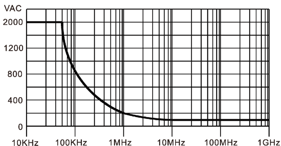
Voltage vs Frequency Rating Curve
