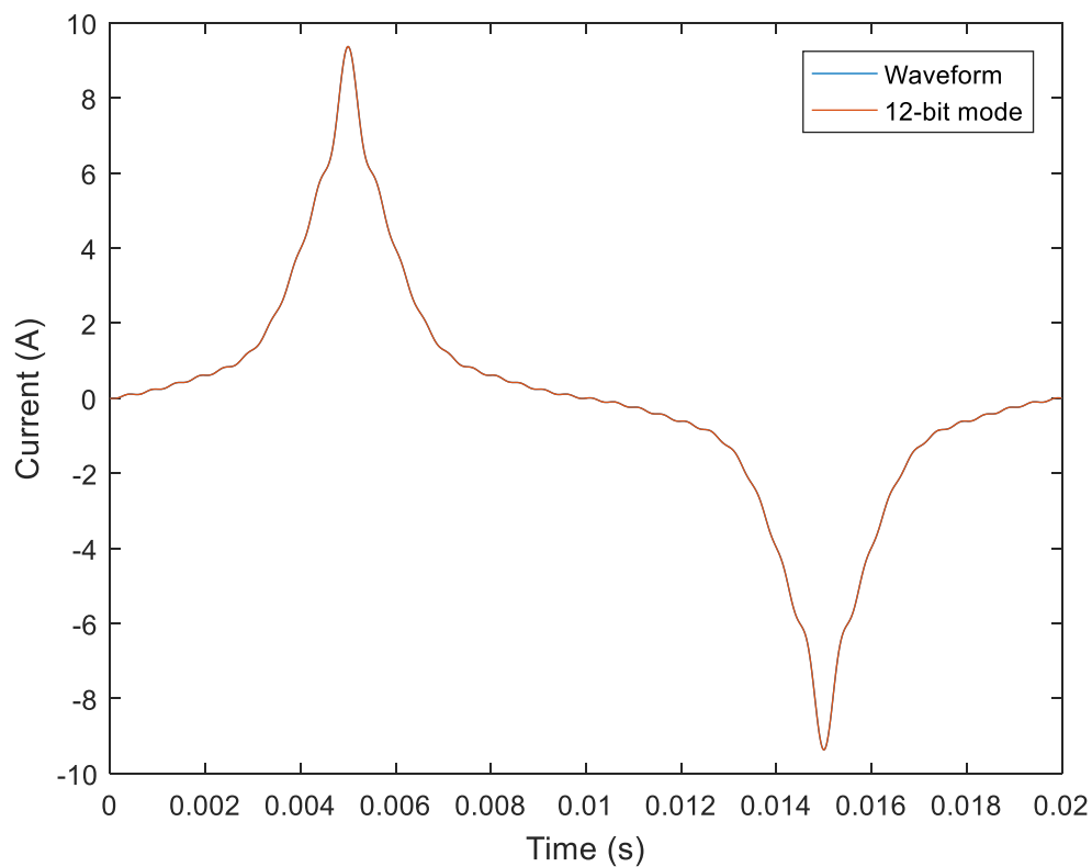
Figure 3: Example IEC waveform with a 50Hz fundamental.
