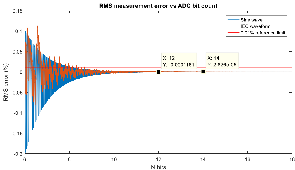
Figure 6: Error is sampled RMS measurement for the IEC and sine waveforms with varying ADC sizes
