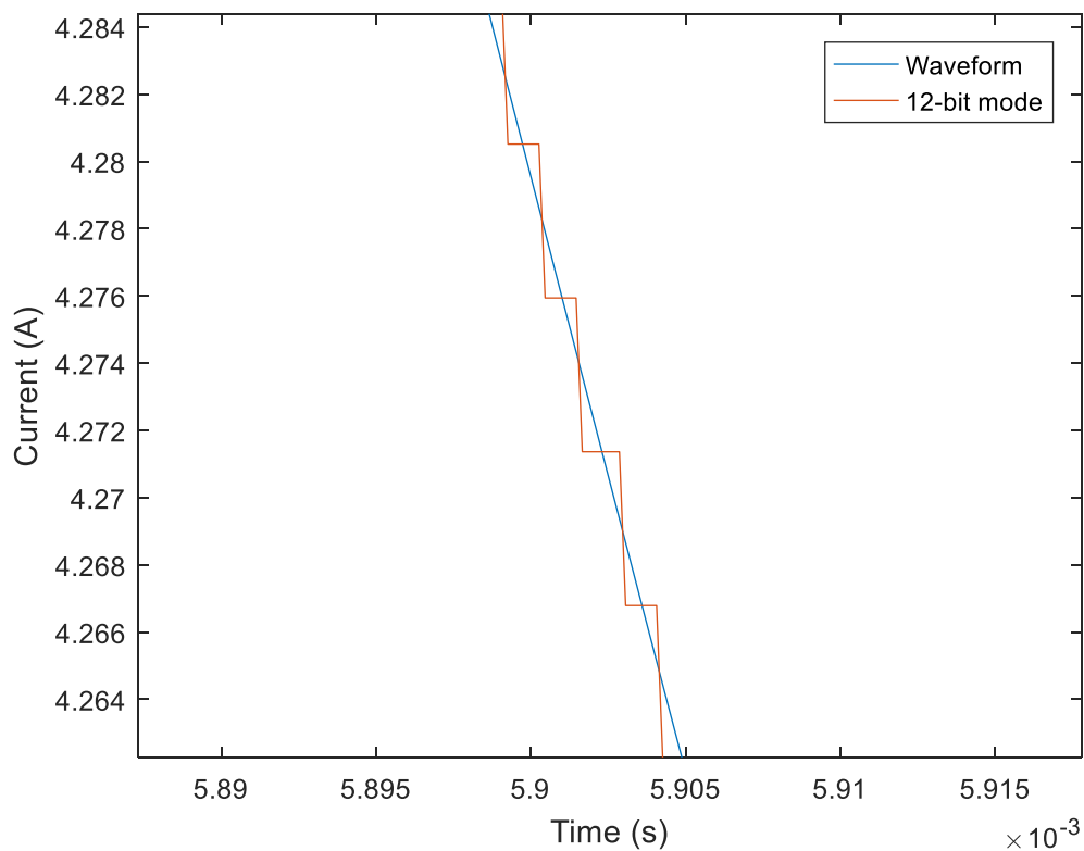
Figure 4: Example IEC waveform - high zoom to show quantisation.
