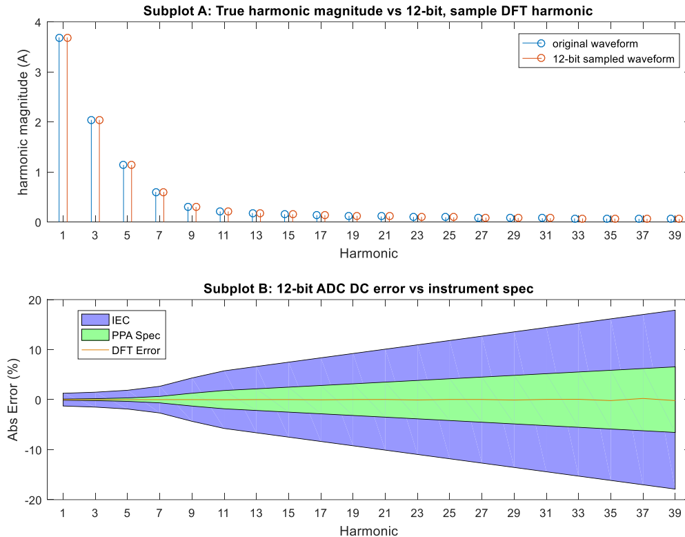
Figure 5: Subplot A: harmonic decomposition of IEC waveform; Subplot B: Magnitude of harmonic error
