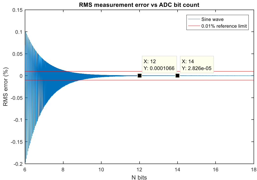
Figure 2: Sampled RMS error vs ADC bit count – 0.01% error shown for reference
